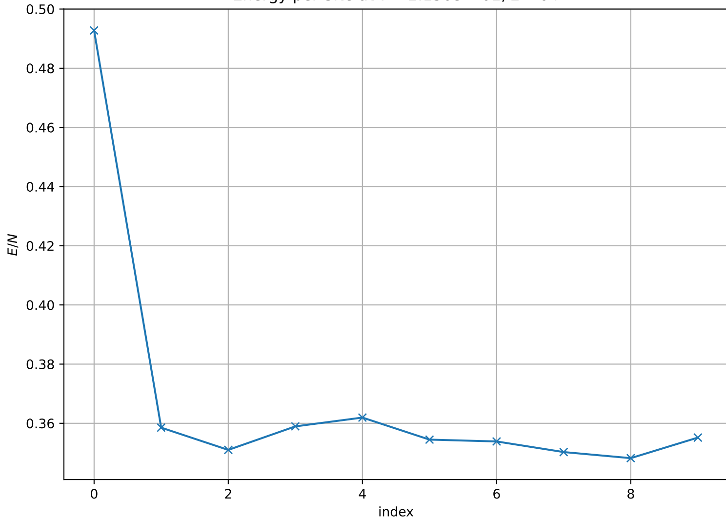
Energy per Site at T = 2.150e - 01 , L = 64
