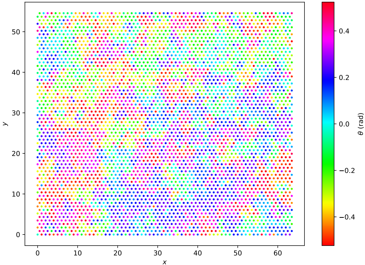
Hexagonal Lattice L=64 , T = 2.15e - 01
