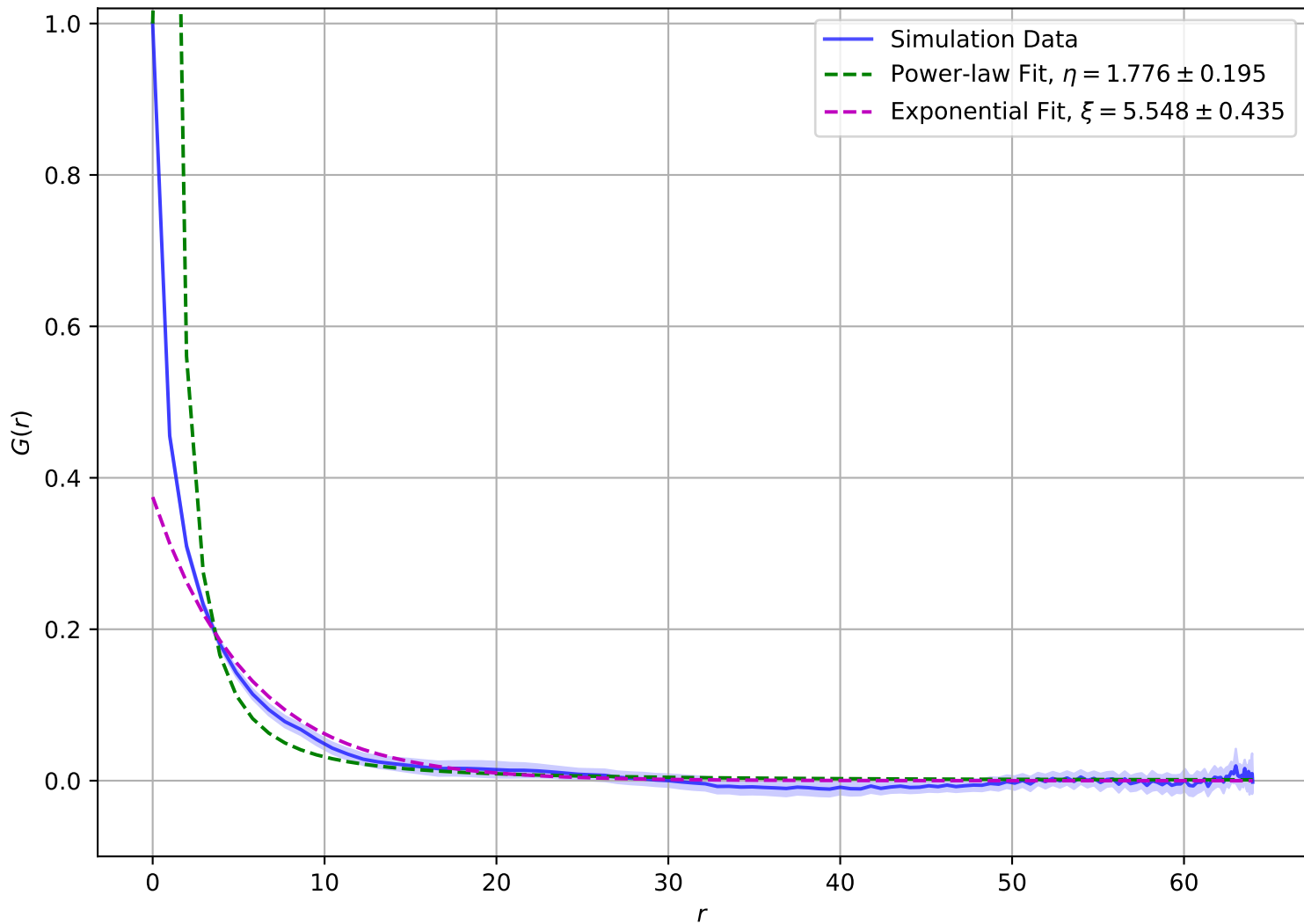
Correlation Function at T = 2.20e - 01 , L = 64
