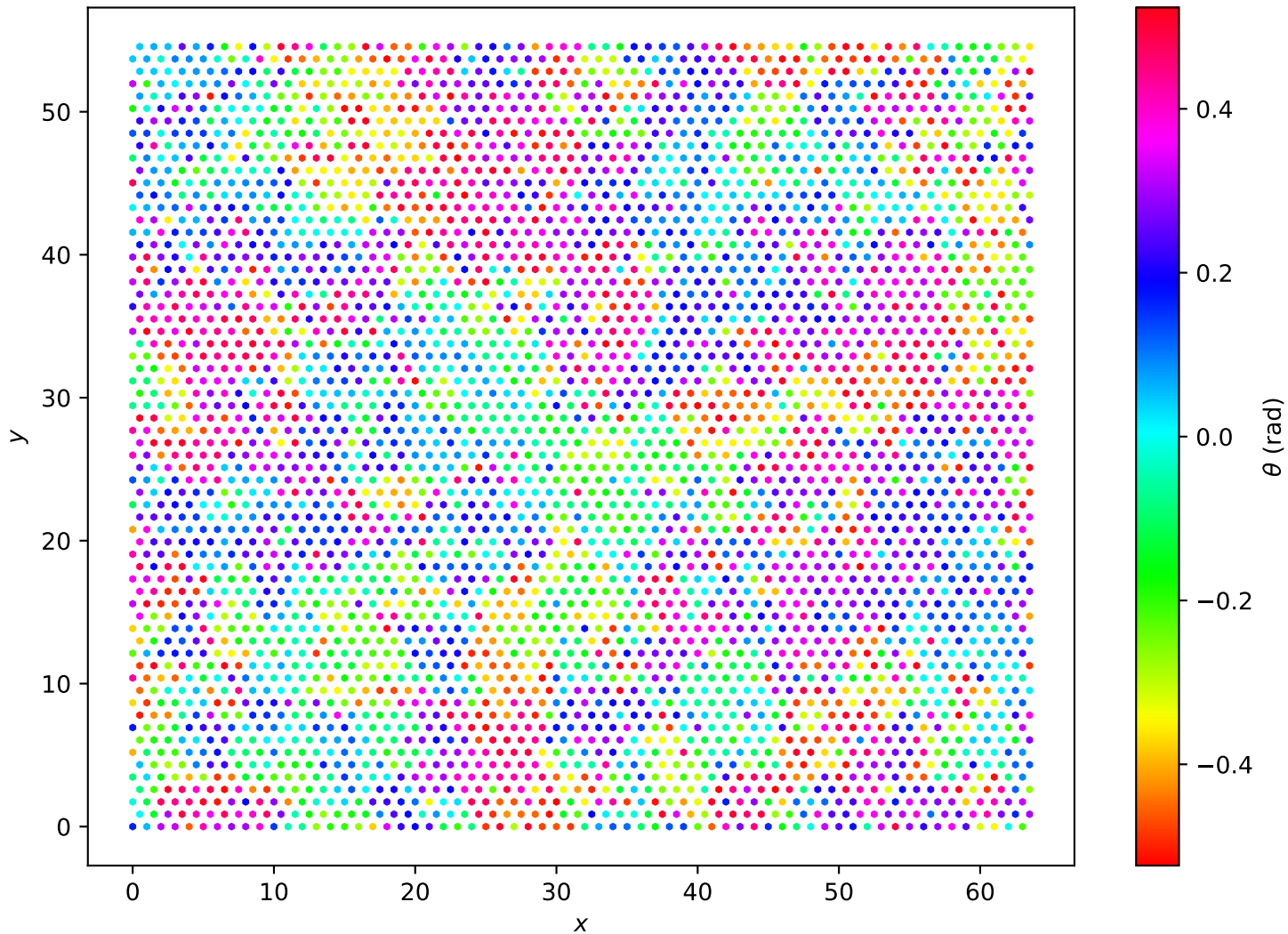
Hexagonal Lattice L=64 , T = 2.20e - 01
