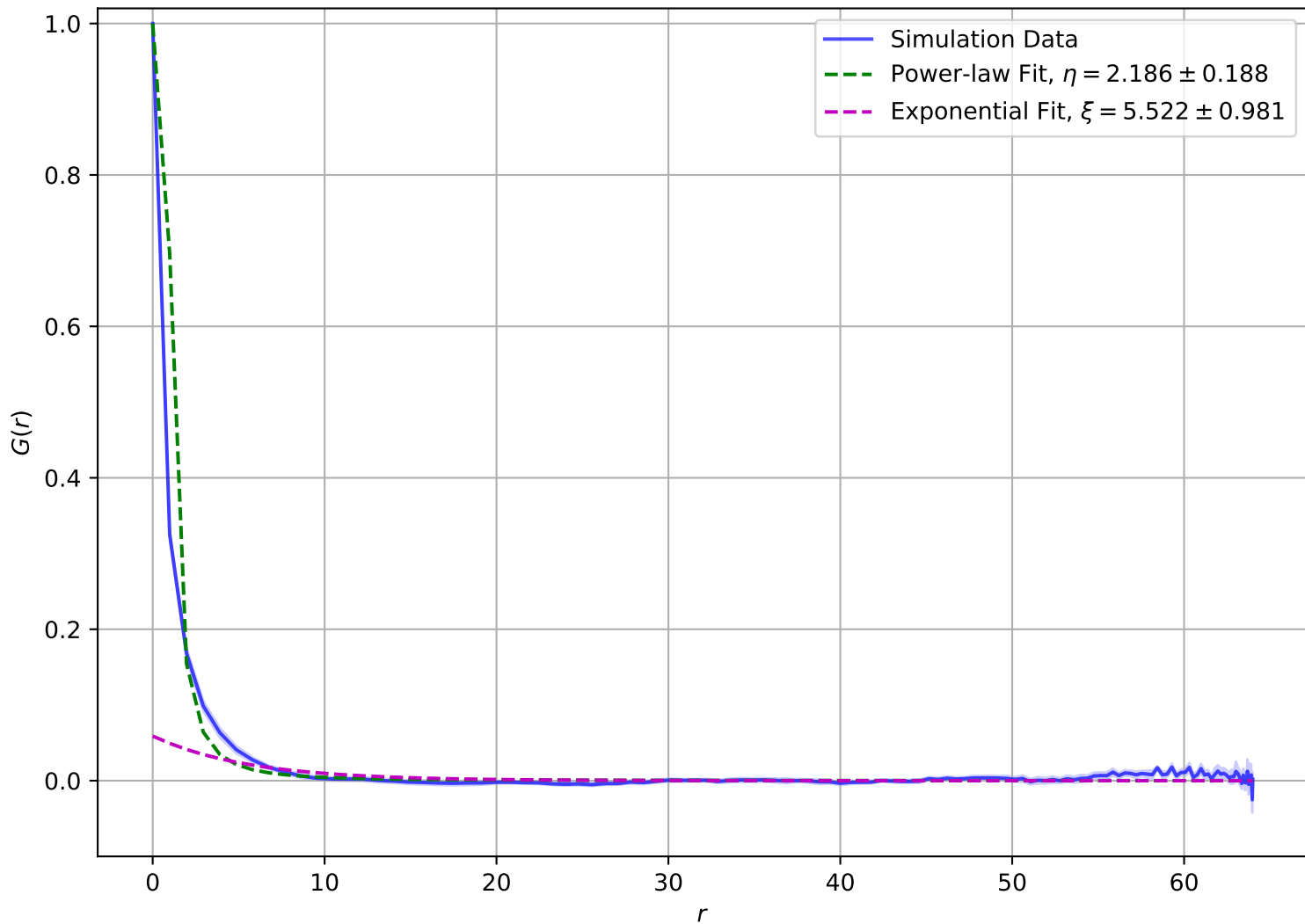
Correlation Function at T = 2.50e - 01 , L = 64
