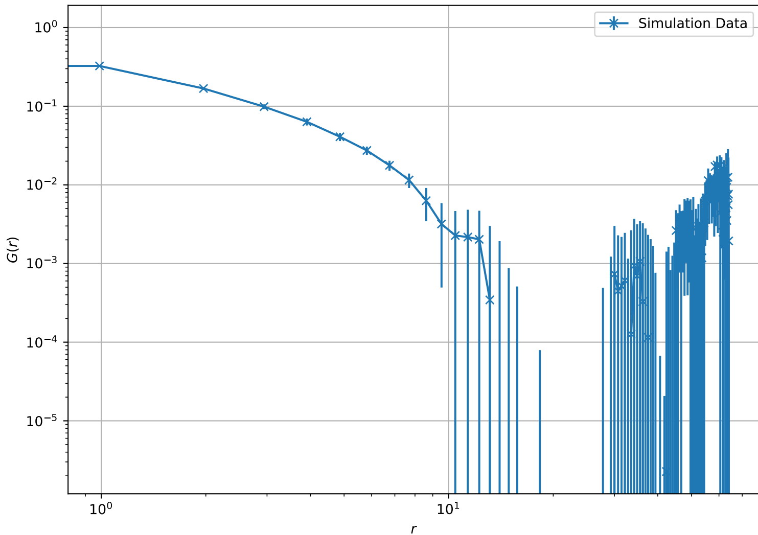
Correlation Function at T = 2.50e - 01 , L = 64 (Log-Log Scale)
