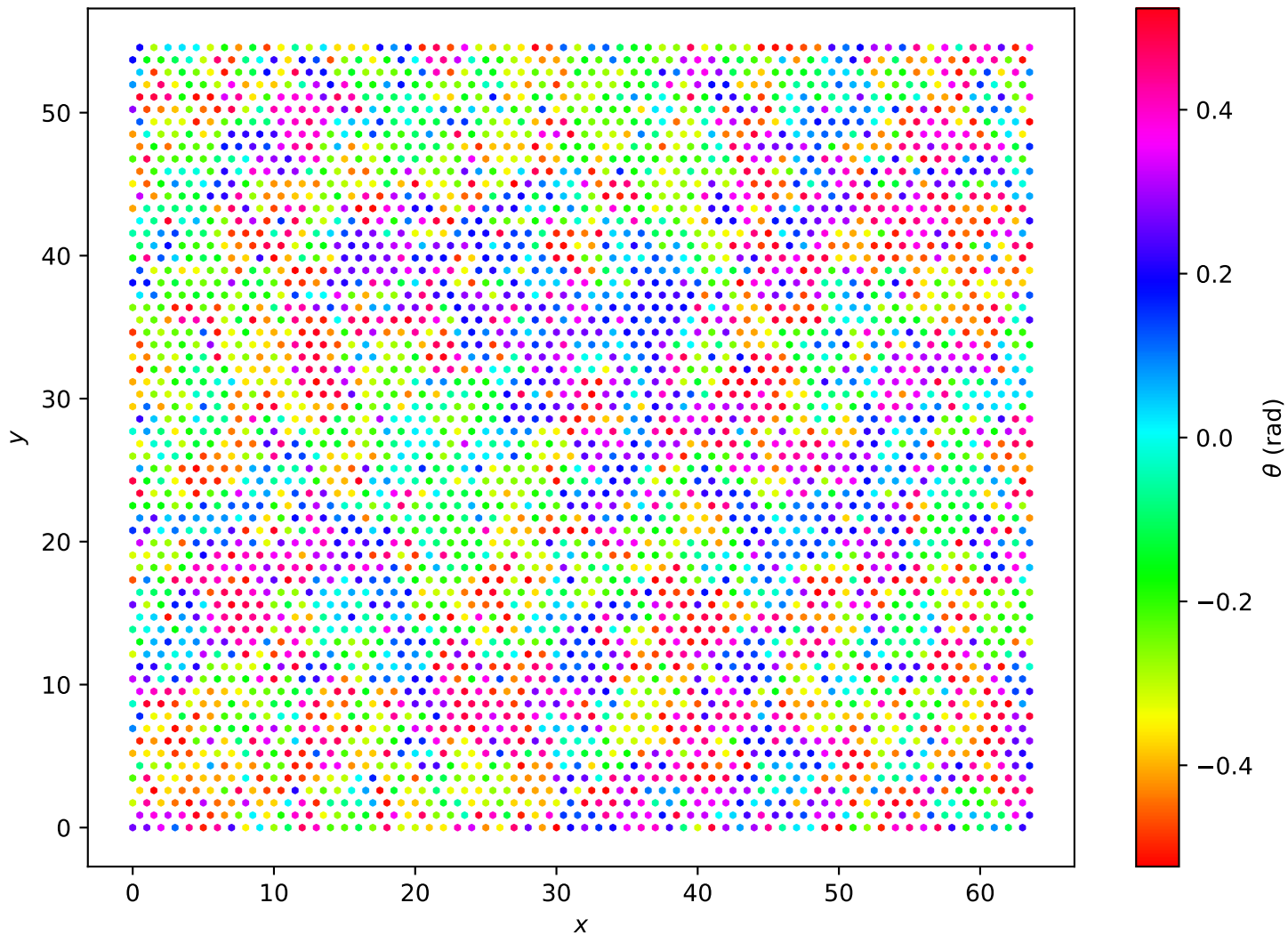
Hexagonal Lattice L=64 , T = 2.50e - 01
