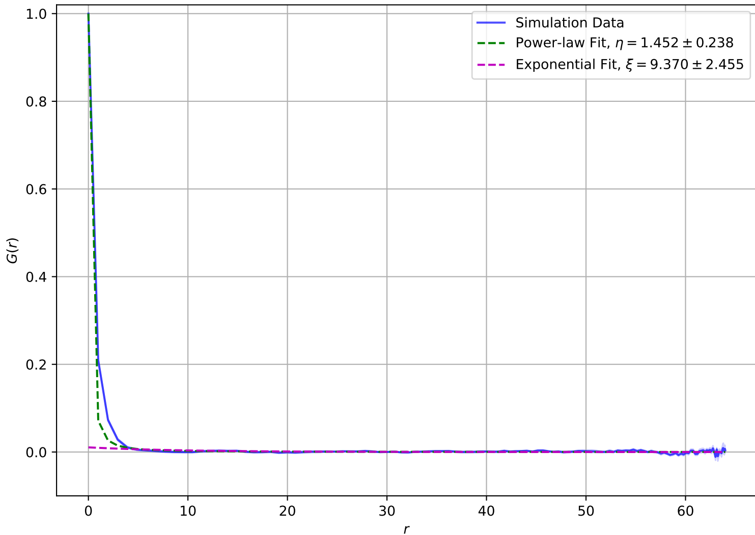
Correlation Function at T = 3.00e - 01 , L = 64
