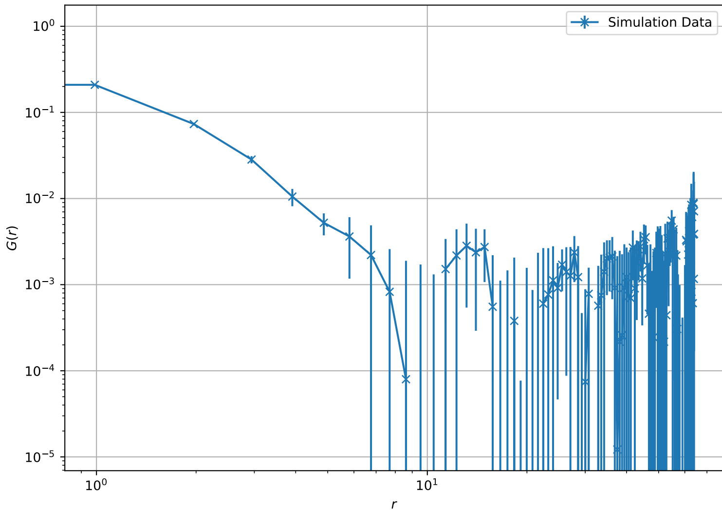
Correlation Function at T = 3.00e - 01 , L = 64 (Log-Log Scale)
