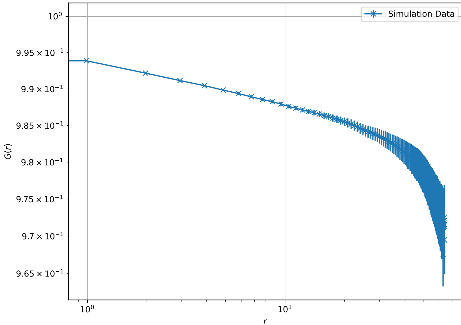
Correlation Function at T = 5.00e - 02 , L = 64 (Log-Log Scale)
