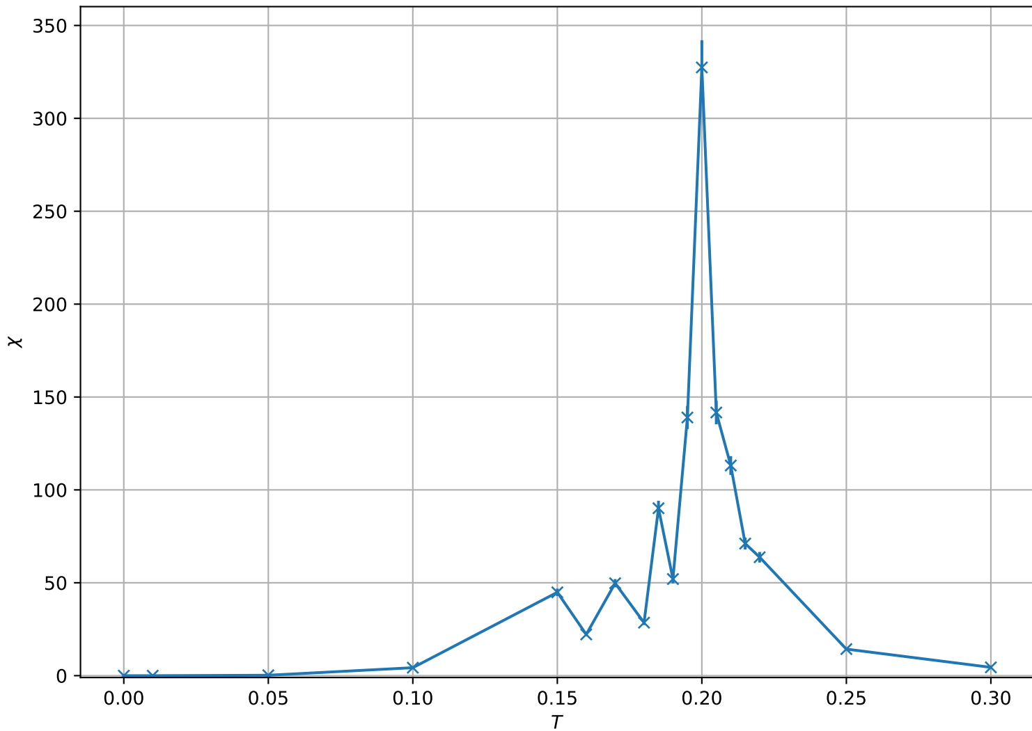
Susceptibility \chi vs Temperature for L = 64
