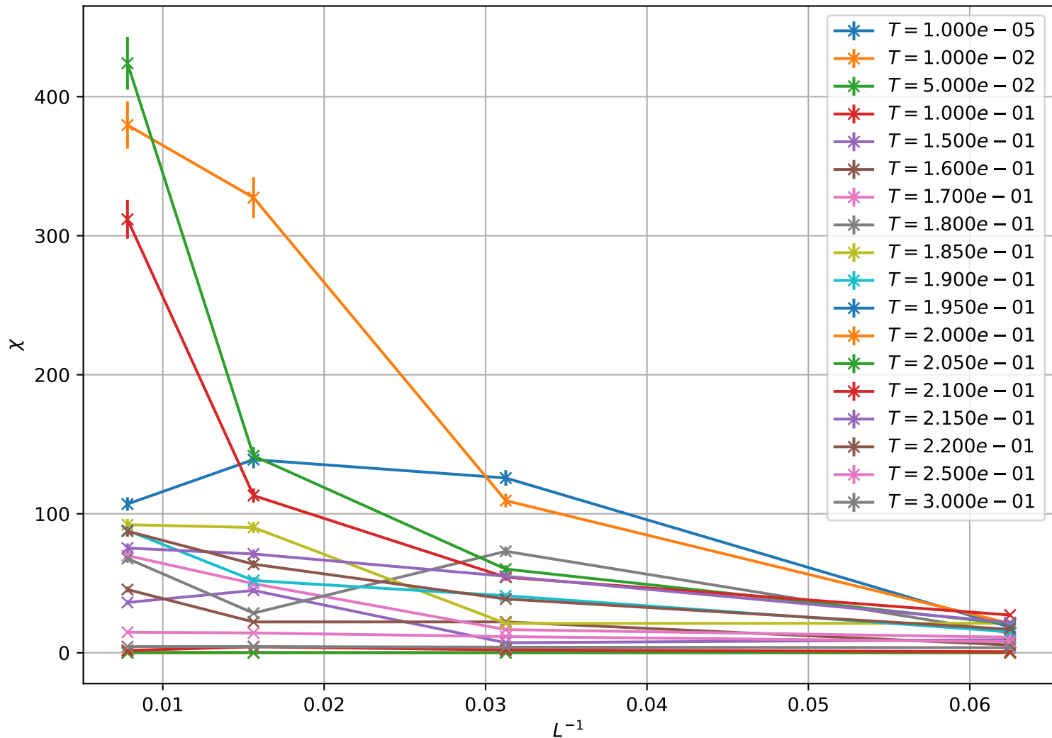
Susceptibility \chi vs System Size L^{-1}
