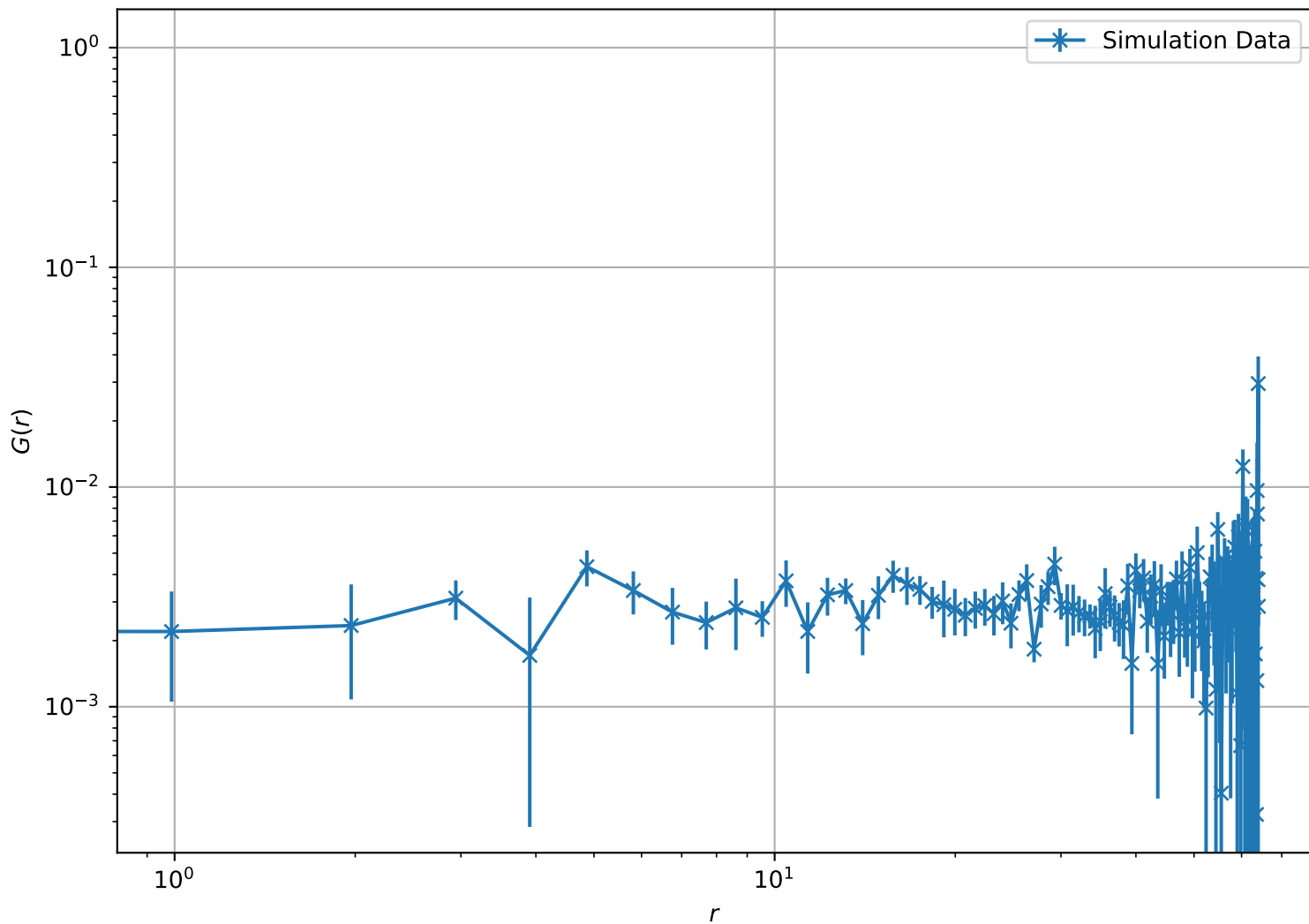
Correlation Function at T = 1.00\text{e} + 00 , L = 64 (Log-Log Scale)
