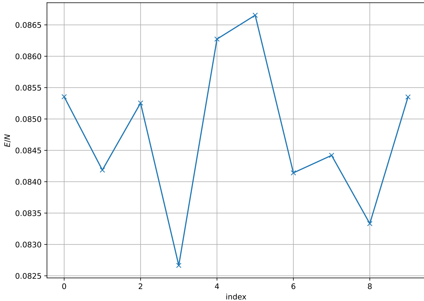
Energy per Site at T = 1.000e + 00 , L = 64
