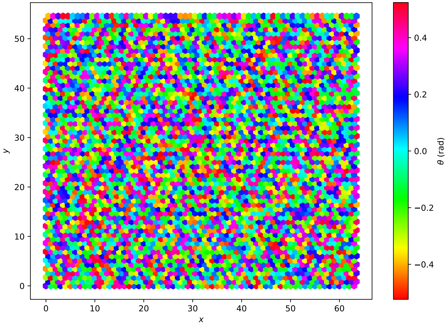
Hexagonal Lattice L=64 , T = 1.00e + 00
