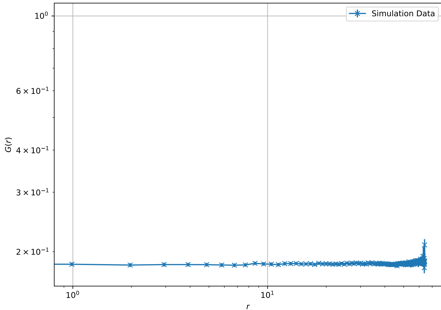
Correlation Function at T = 1.00\text{e} - 01 , L = 64 (Log-Log Scale)
