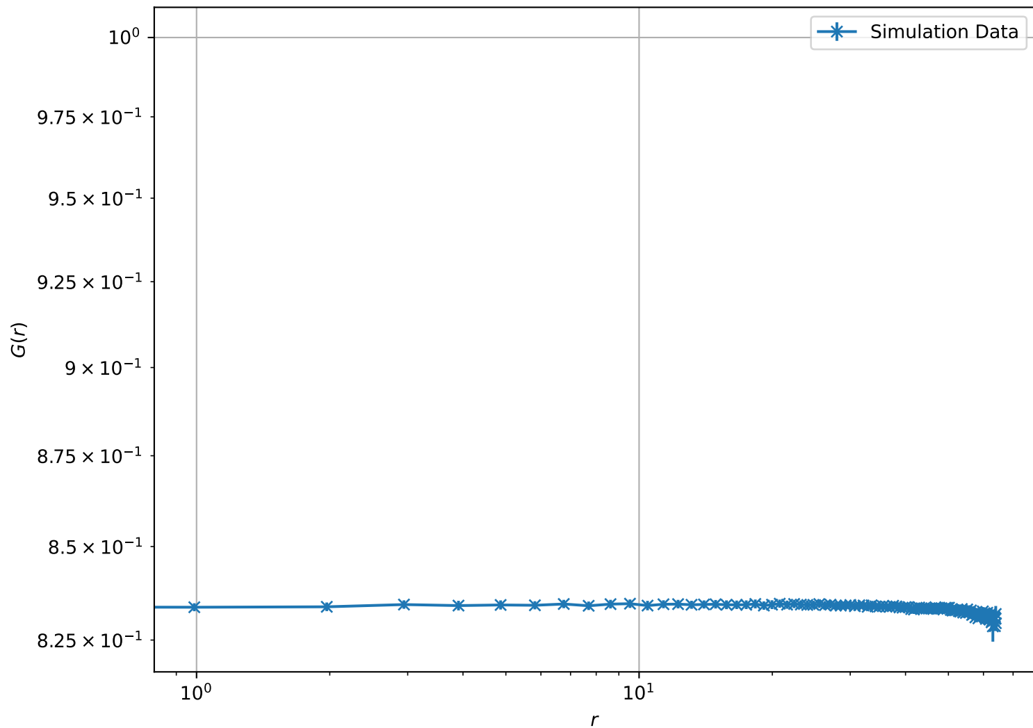
Correlation Function at T = 1.00\text{e} - 02 , L = 64 (Log-Log Scale)
