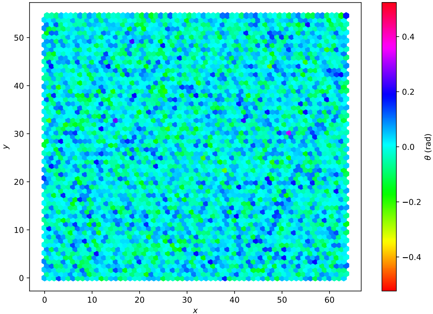
Hexagonal Lattice L=64 , T = 1.00e - 02
