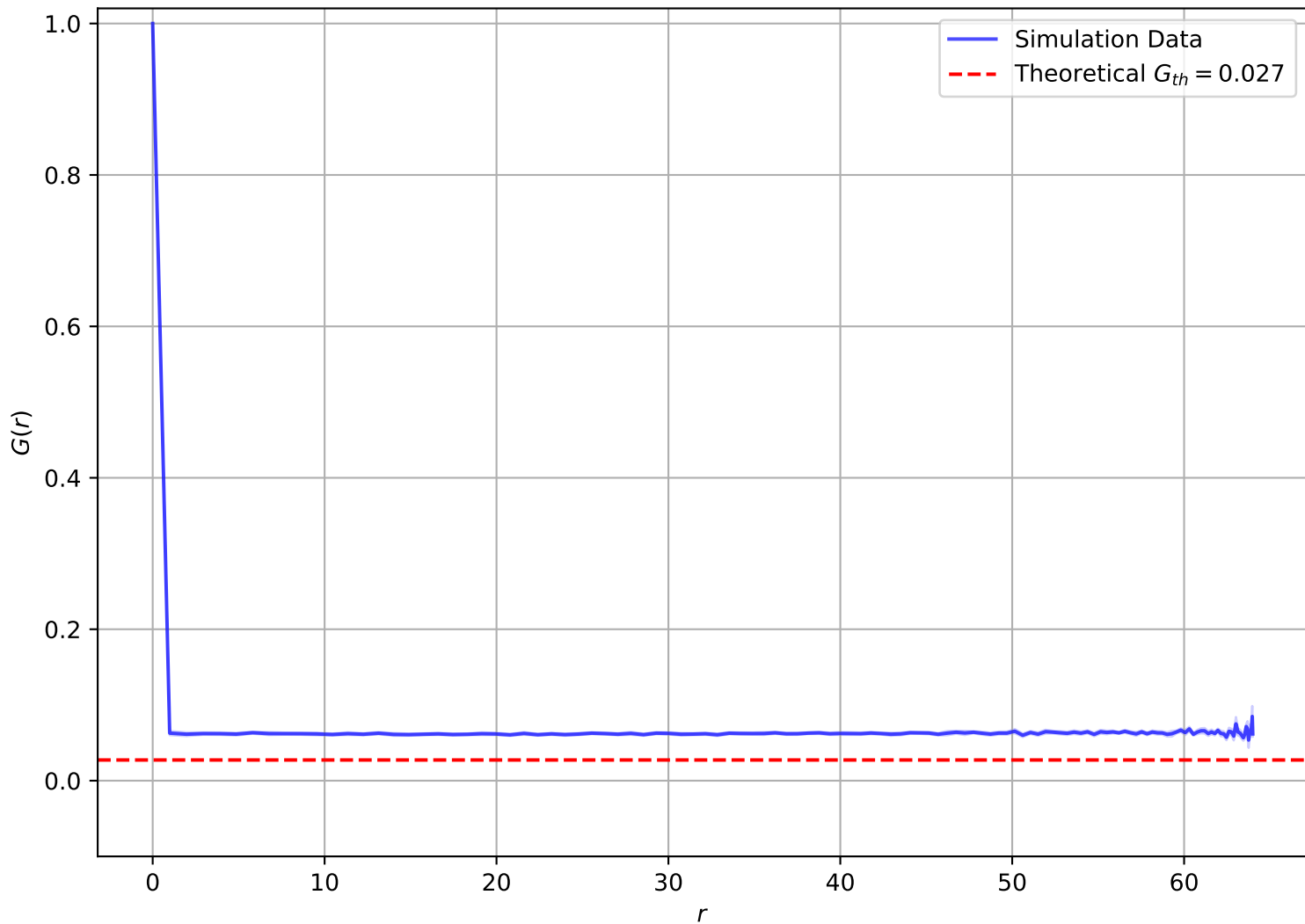
Correlation Function at T = 2.00\text{e} - 01 , L = 64
