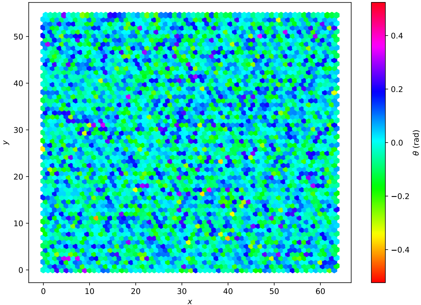
Hexagonal Lattice L=64 , T = 2.50e - 02
