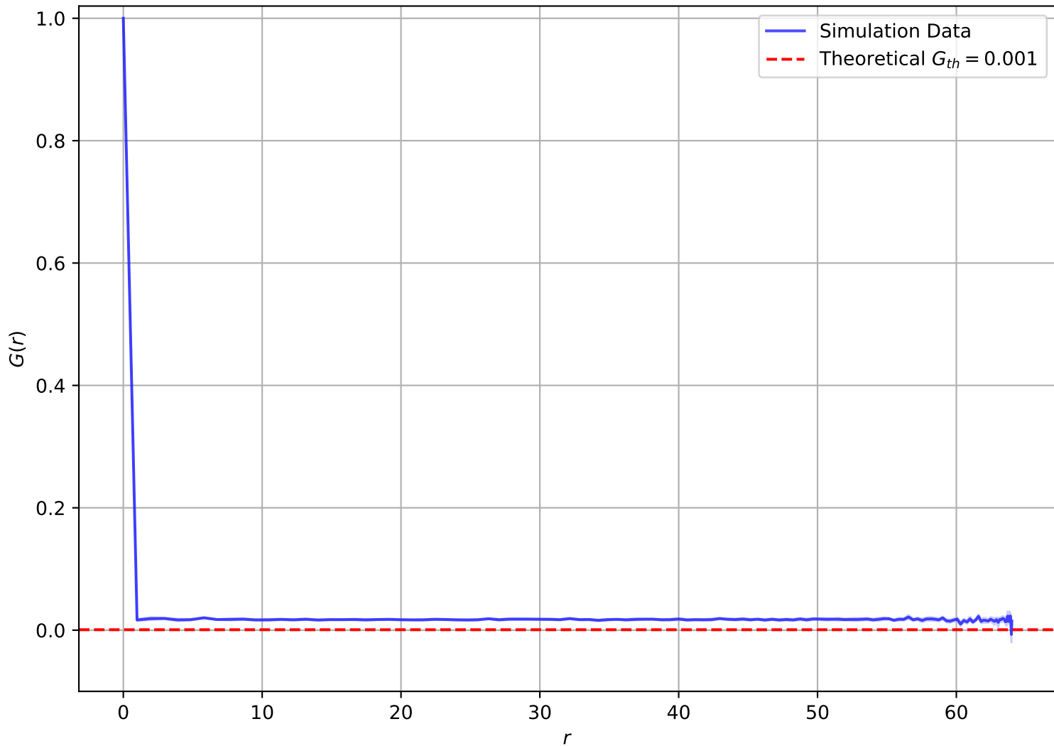
Correlation Function at T = 4.00e - 01 , L = 64
