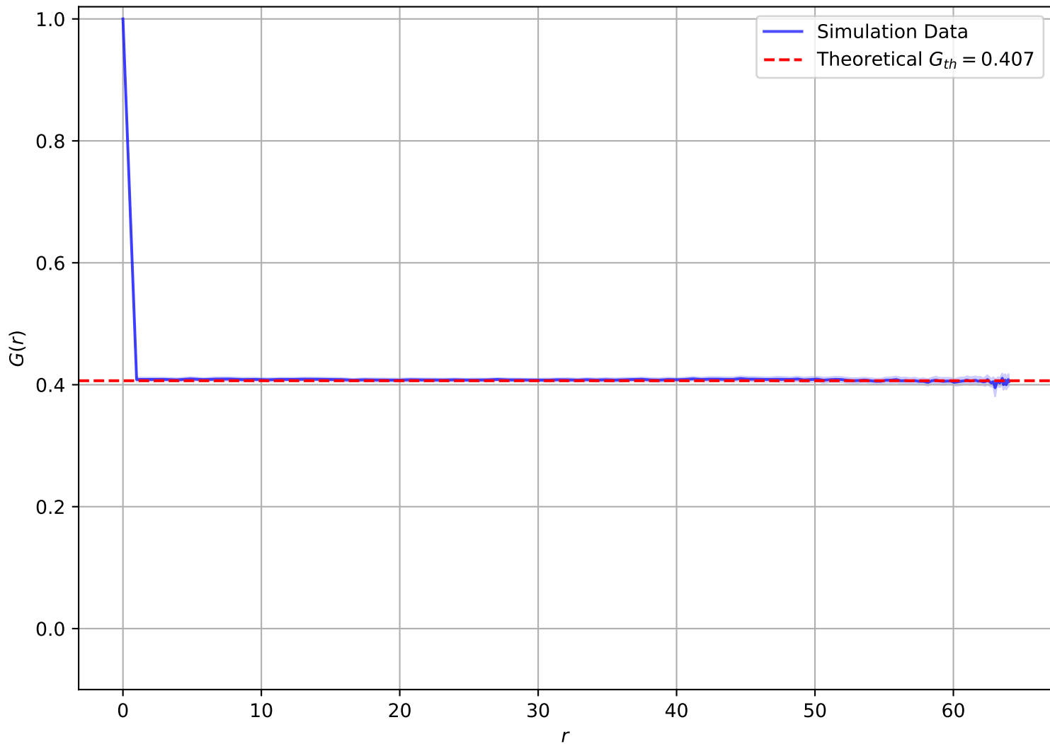
Correlation Function at T = 5.00\text{e} - 02 , L = 64
