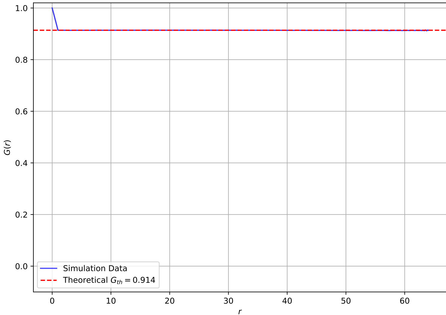
Correlation Function at T = 5.00e - 03 , L = 64
