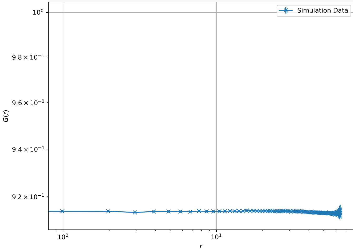
Correlation Function at T = 5.00\text{e} - 03 , L = 64 (Log-Log Scale)
