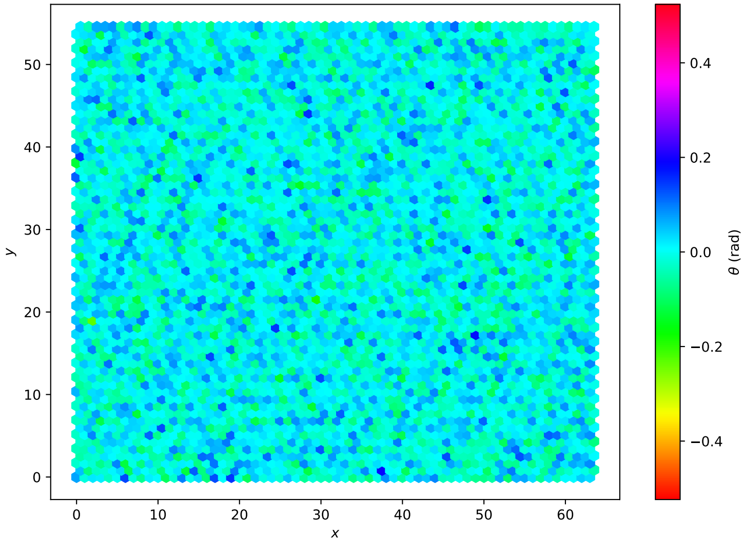
Hexagonal Lattice L=64 , T = 5.00e - 03
