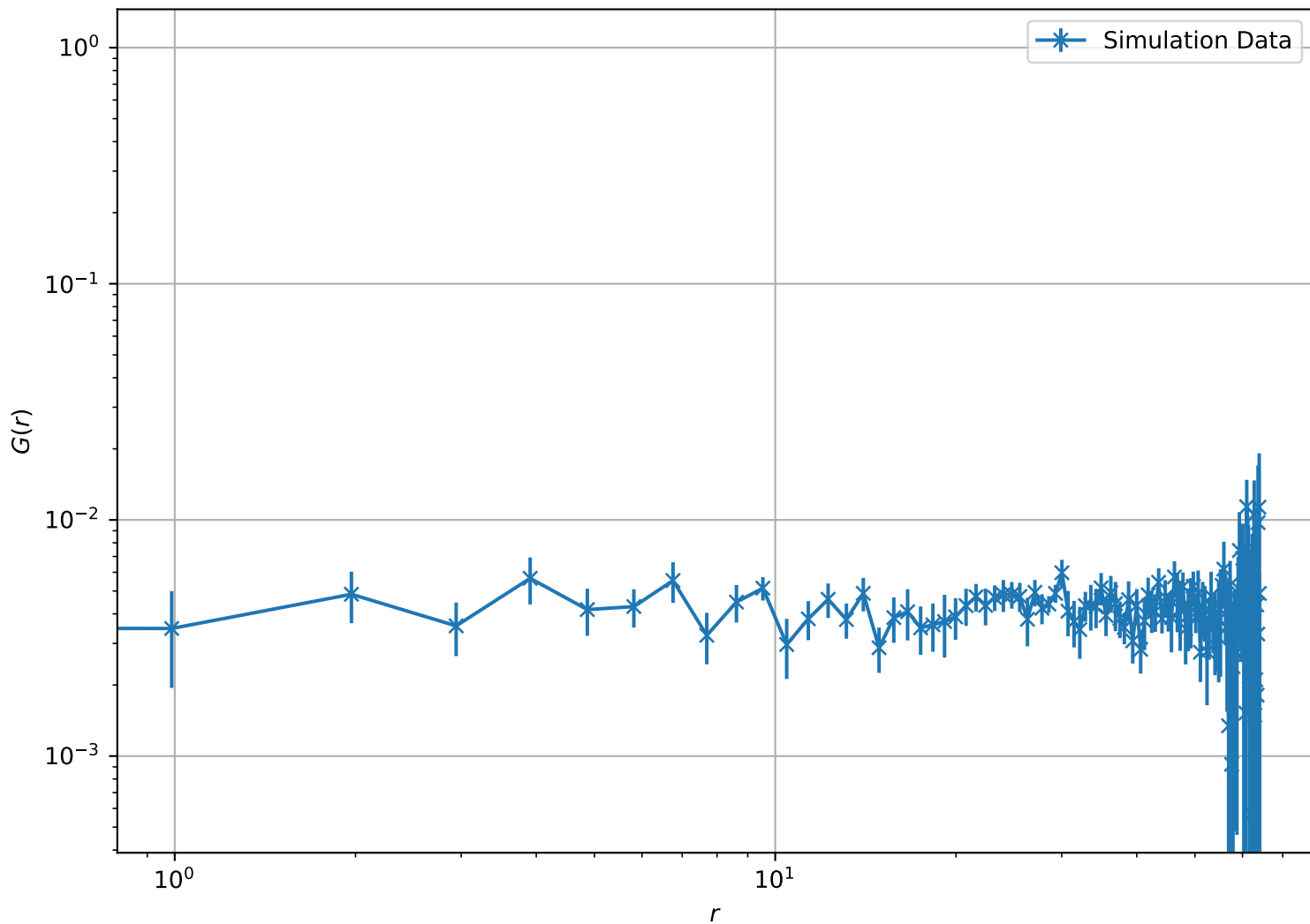
Correlation Function at T = 8.00e - 01 , L = 64 (Log-Log Scale)
