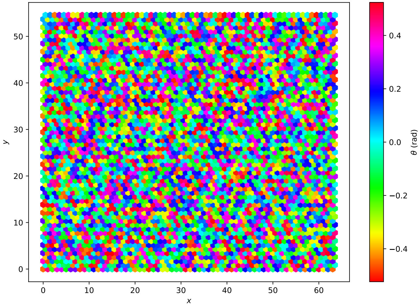
Hexagonal Lattice L=64 , T = 8.00e - 01
