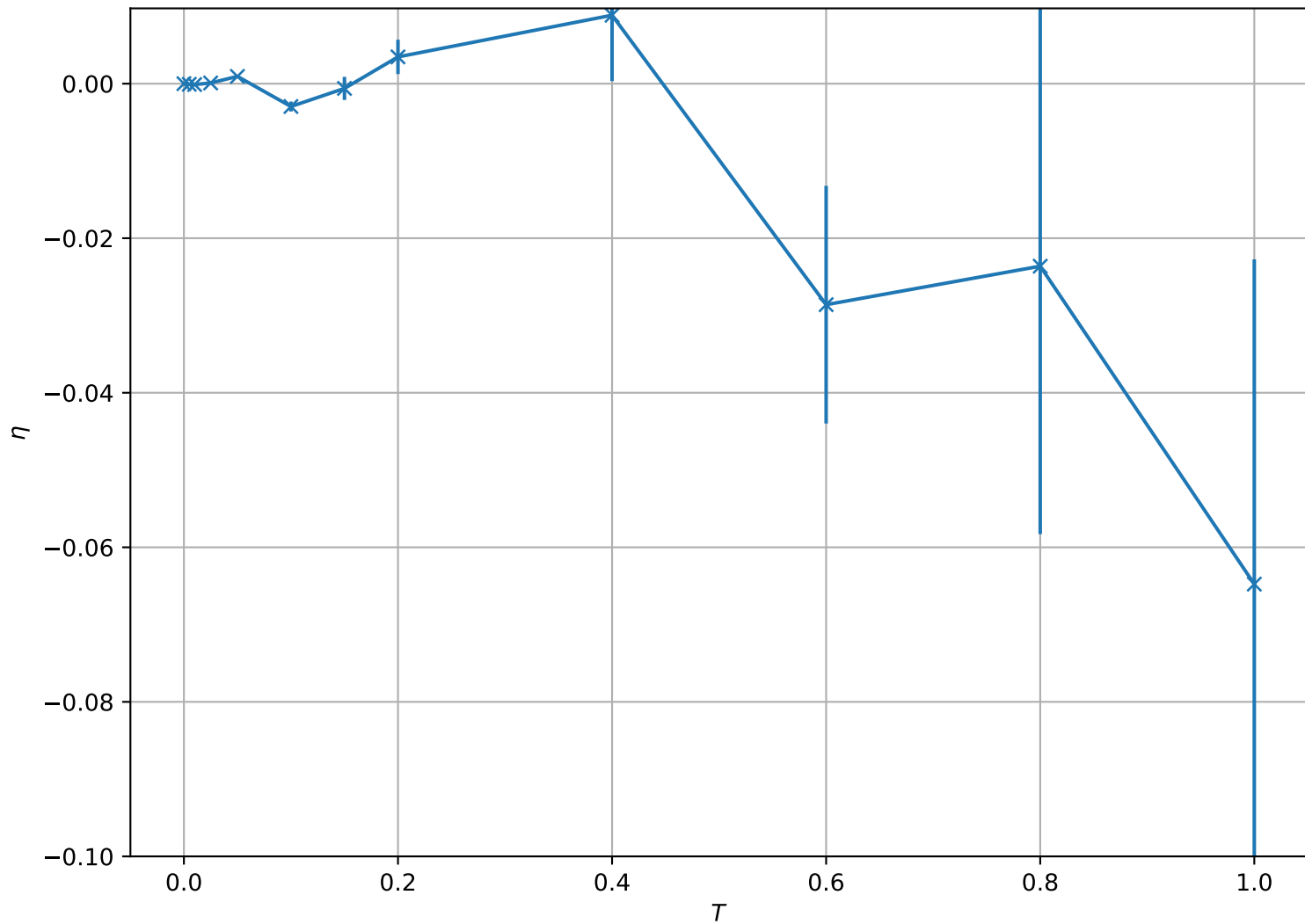
Critical Exponent \eta vs Temperature for L = 64
