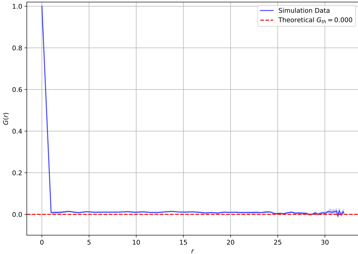
Correlation Function at T = 1.00\text{e} + 00 , L = 32
