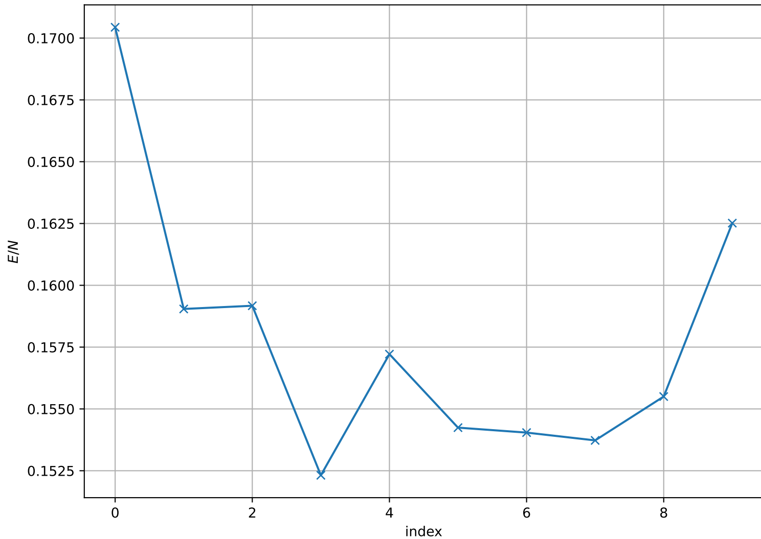
Energy per Site at T = 1.000e + 00 , L = 32
