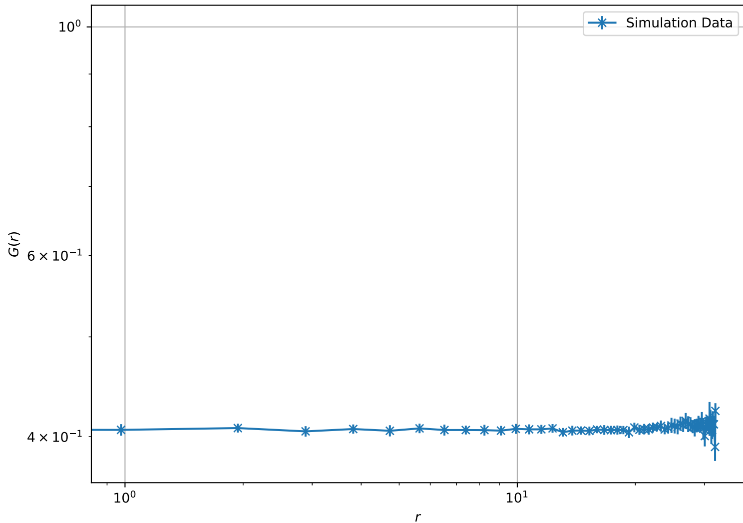
Correlation Function at T = 1.00e - 01 , L = 32 (Log-Log Scale)
