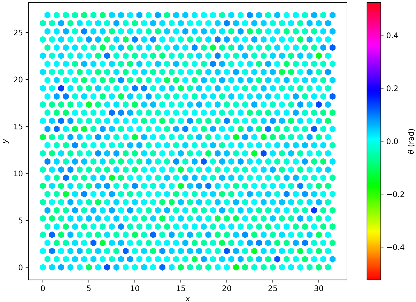
Hexagonal Lattice L=32 , T = 1.00e - 02
