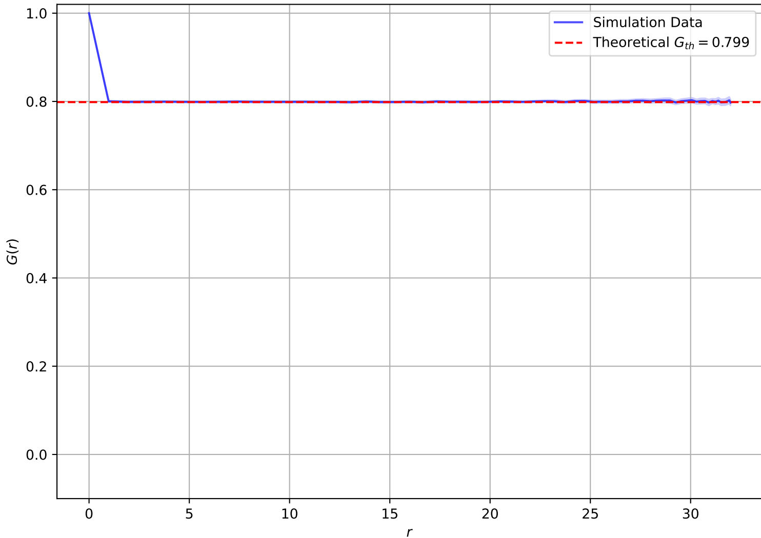
Correlation Function at T = 2.50e - 02 , L = 32
