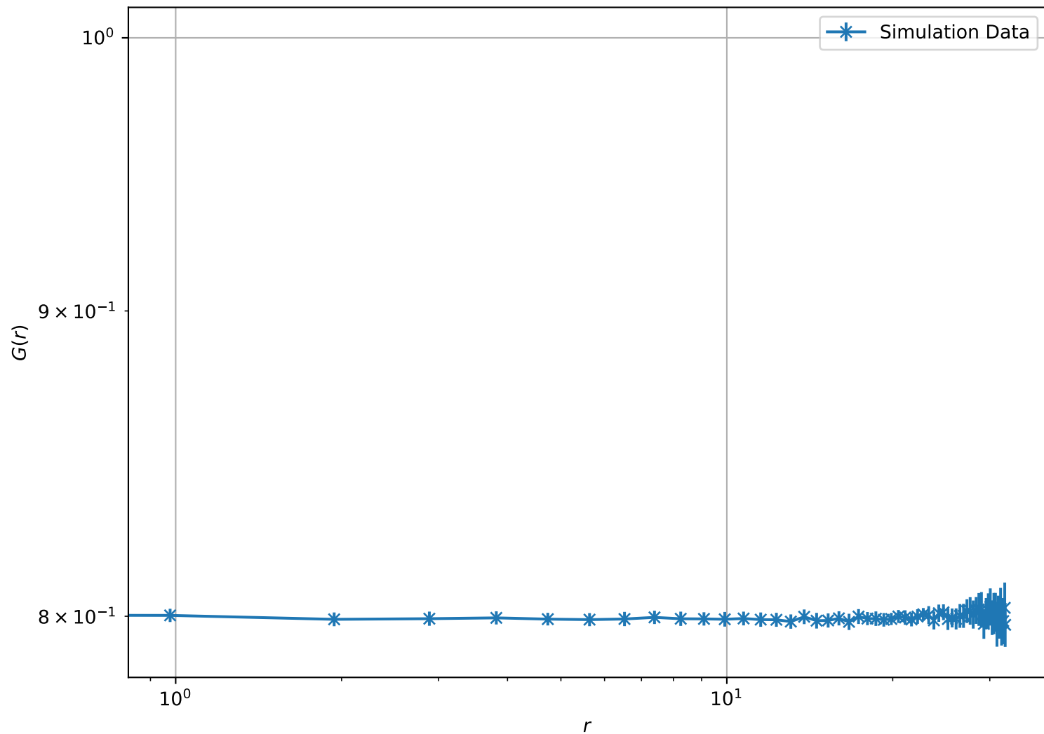
Correlation Function at T = 2.50e - 02 , L = 32 (Log-Log Scale)
