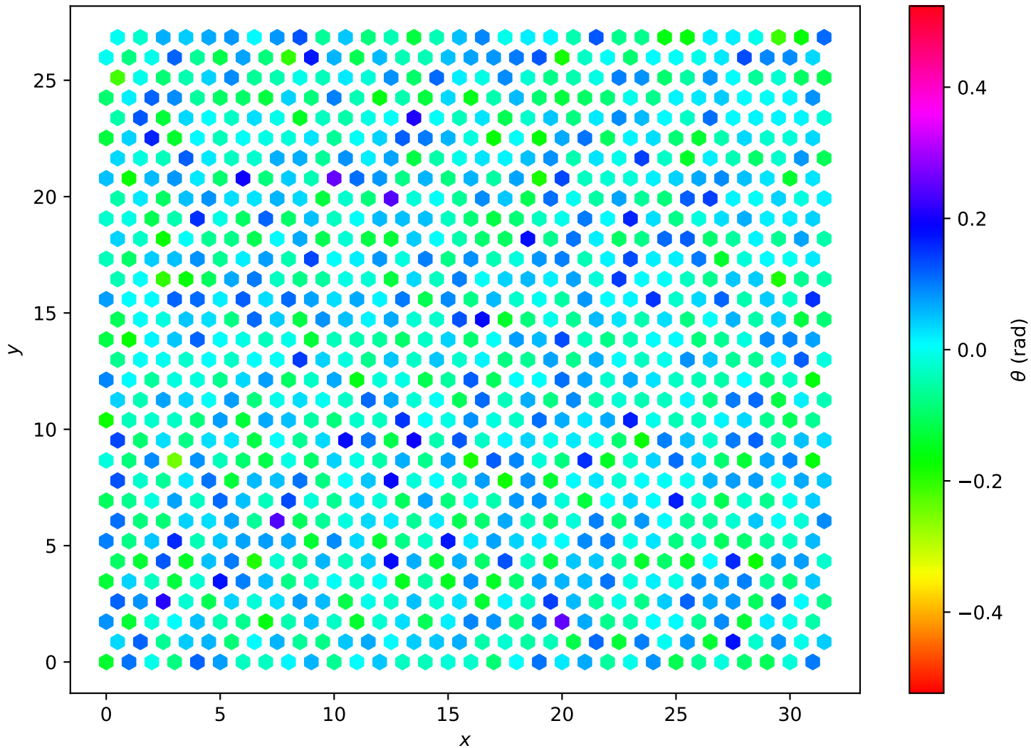
Hexagonal Lattice L=32 , T = 2.50e - 02
