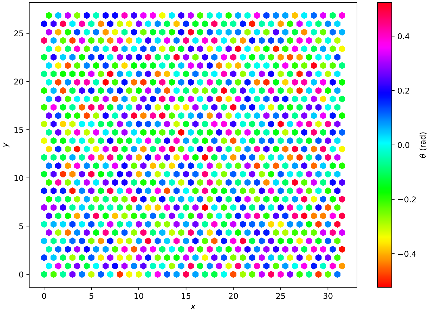
Hexagonal Lattice L=32 , T = 4.00e - 01
