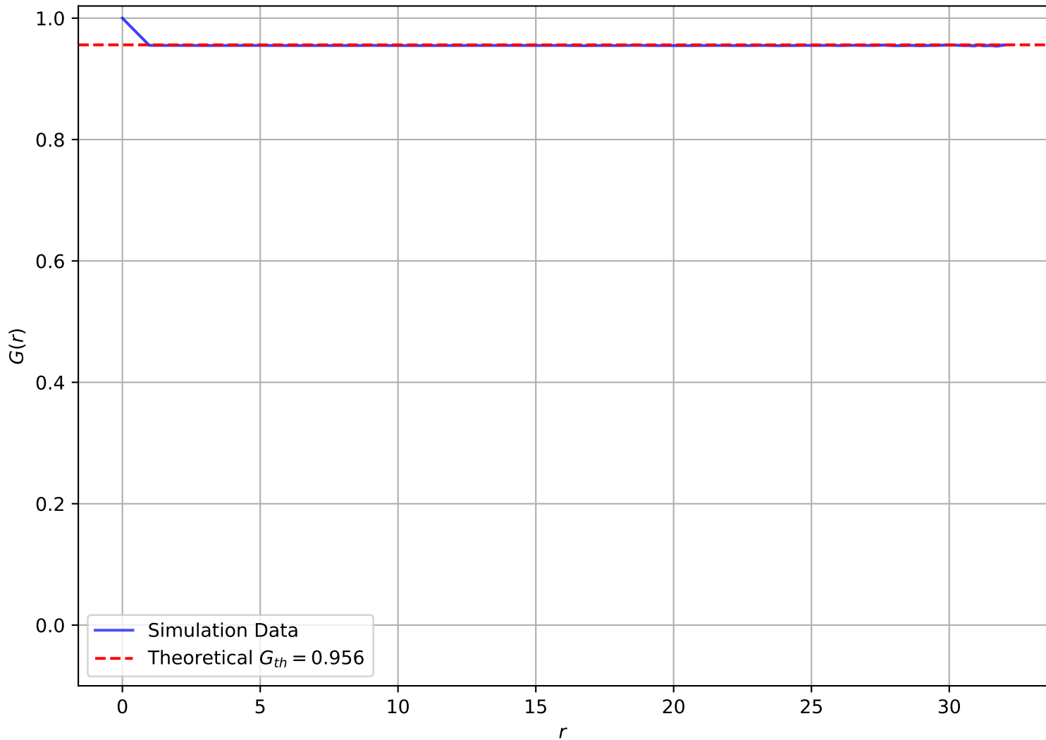
Correlation Function at T = 5.00e - 03 , L = 32
