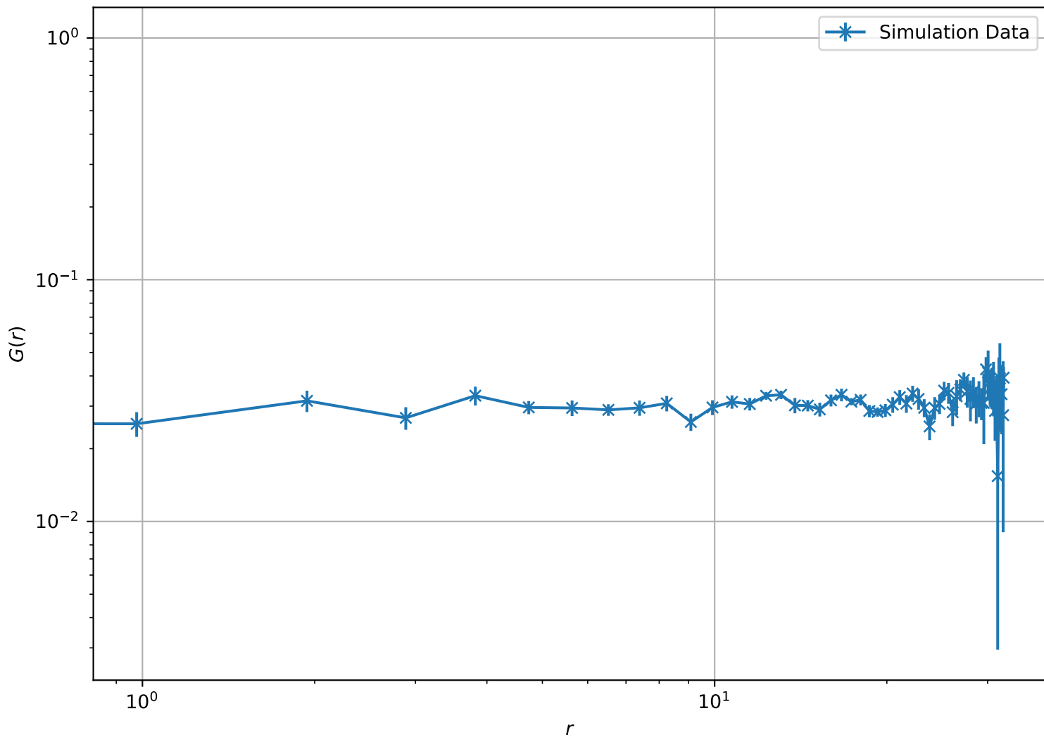
Correlation Function at T = 6.00e - 01 , L = 32 (Log-Log Scale)
