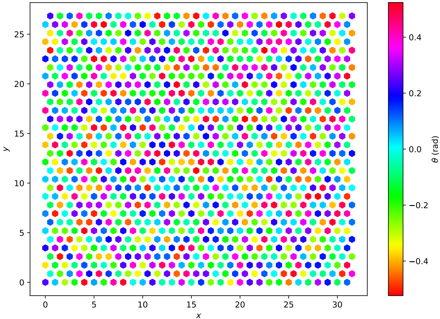
Hexagonal Lattice L=32 , T = 8.00e - 01
