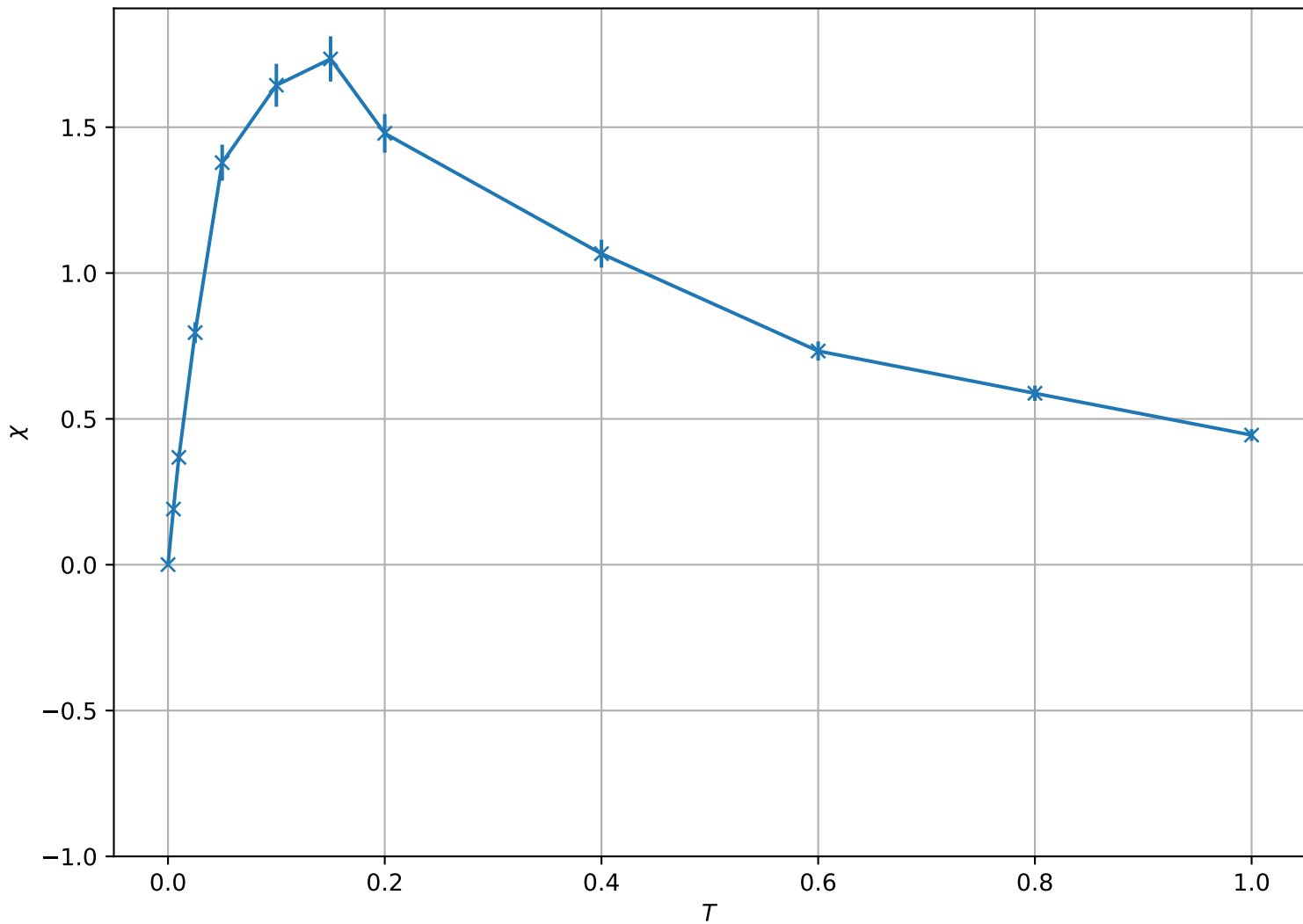
Susceptibility \chi vs Temperature for L = 32
