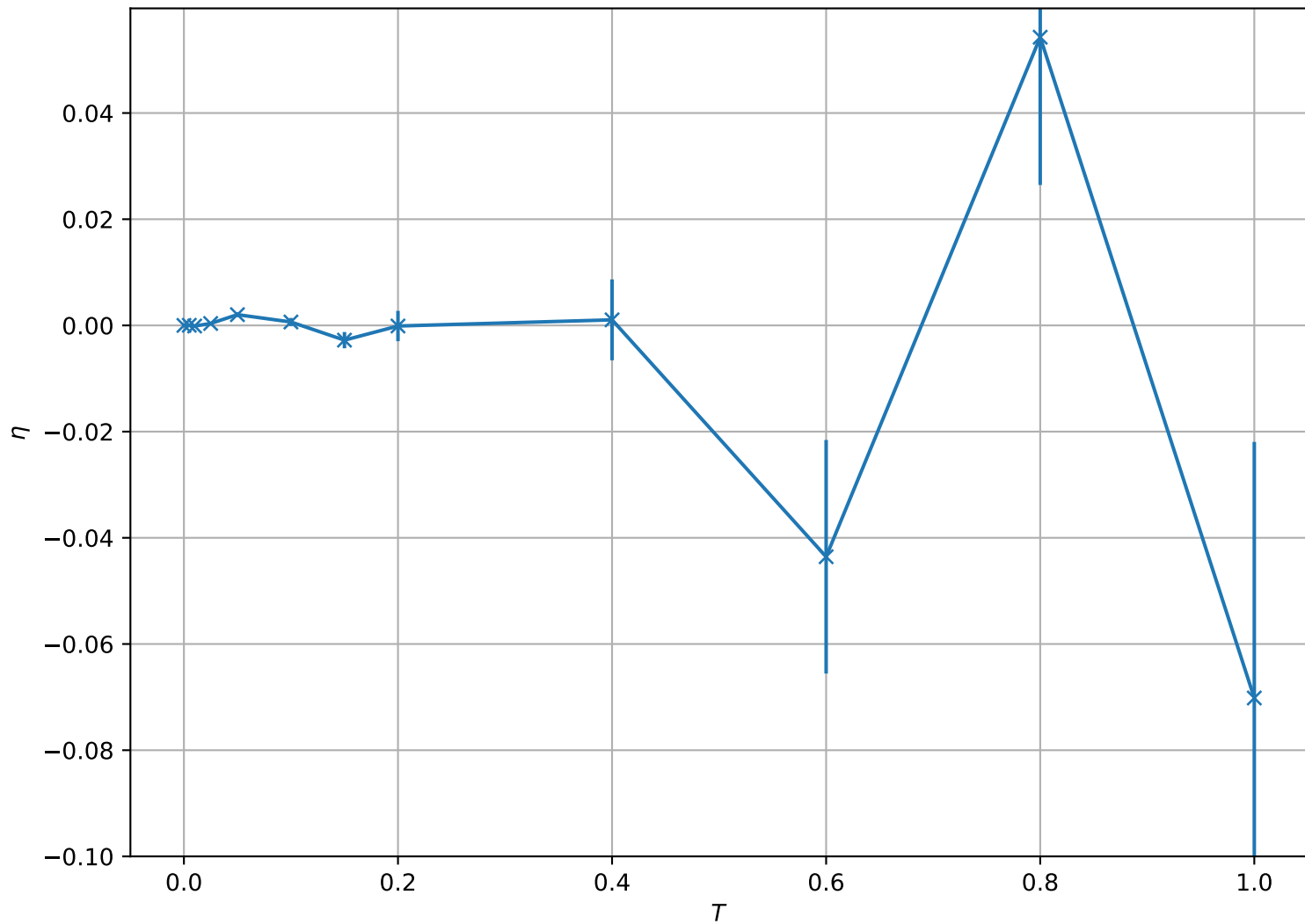
Critical Exponent \eta vs Temperature for L = 32
