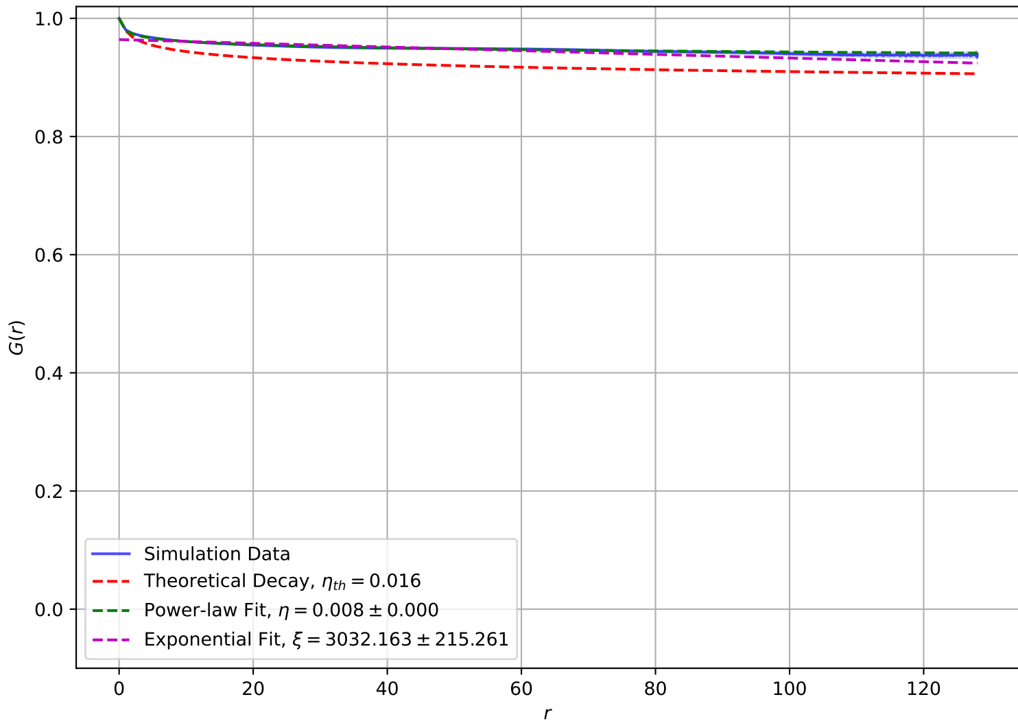
Correlation Function at T = 1.00\text{e} - 01 , L = 128
