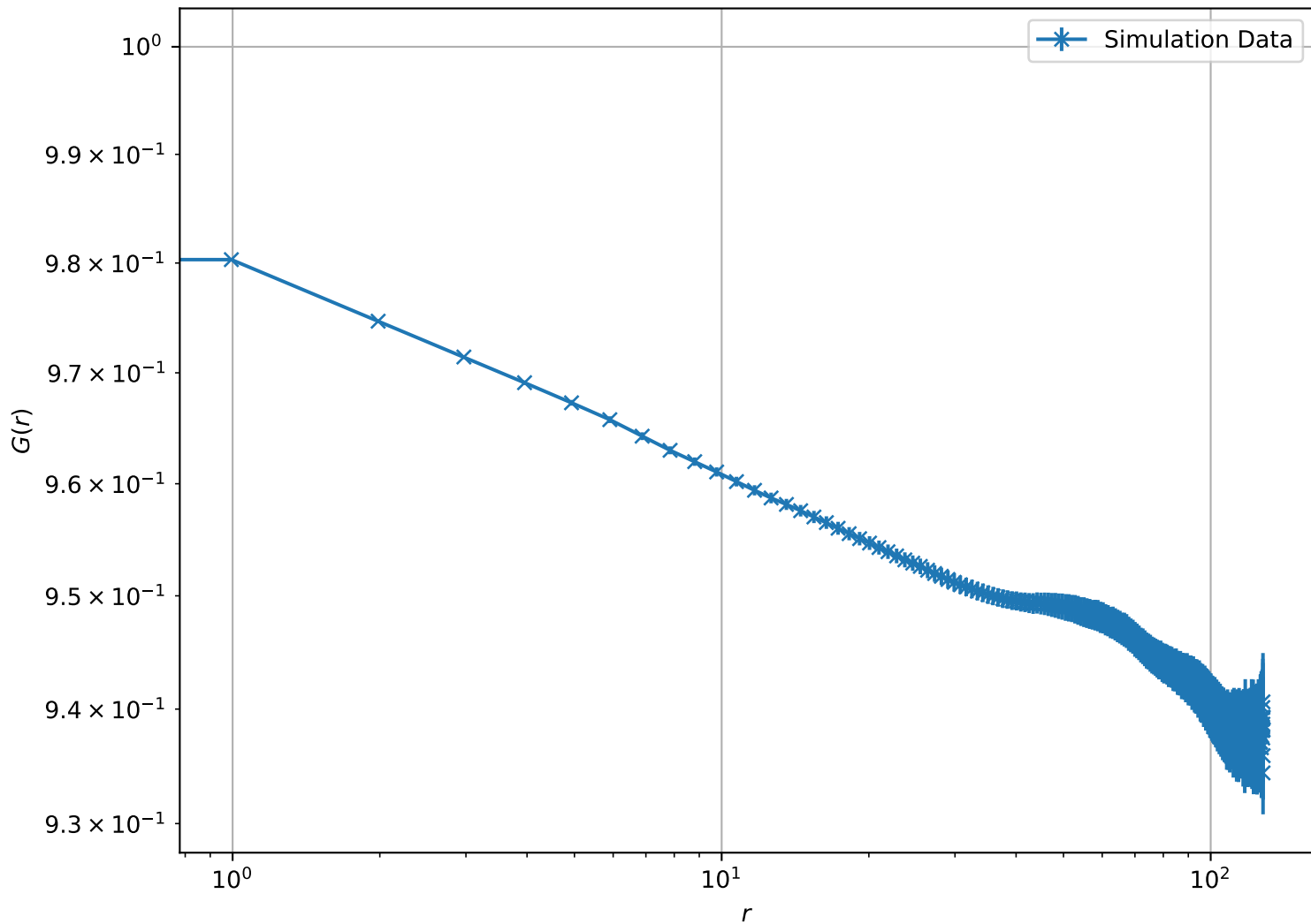
Correlation Function at T = 1.00\text{e} - 01 , L = 128 (Log-Log Scale)
