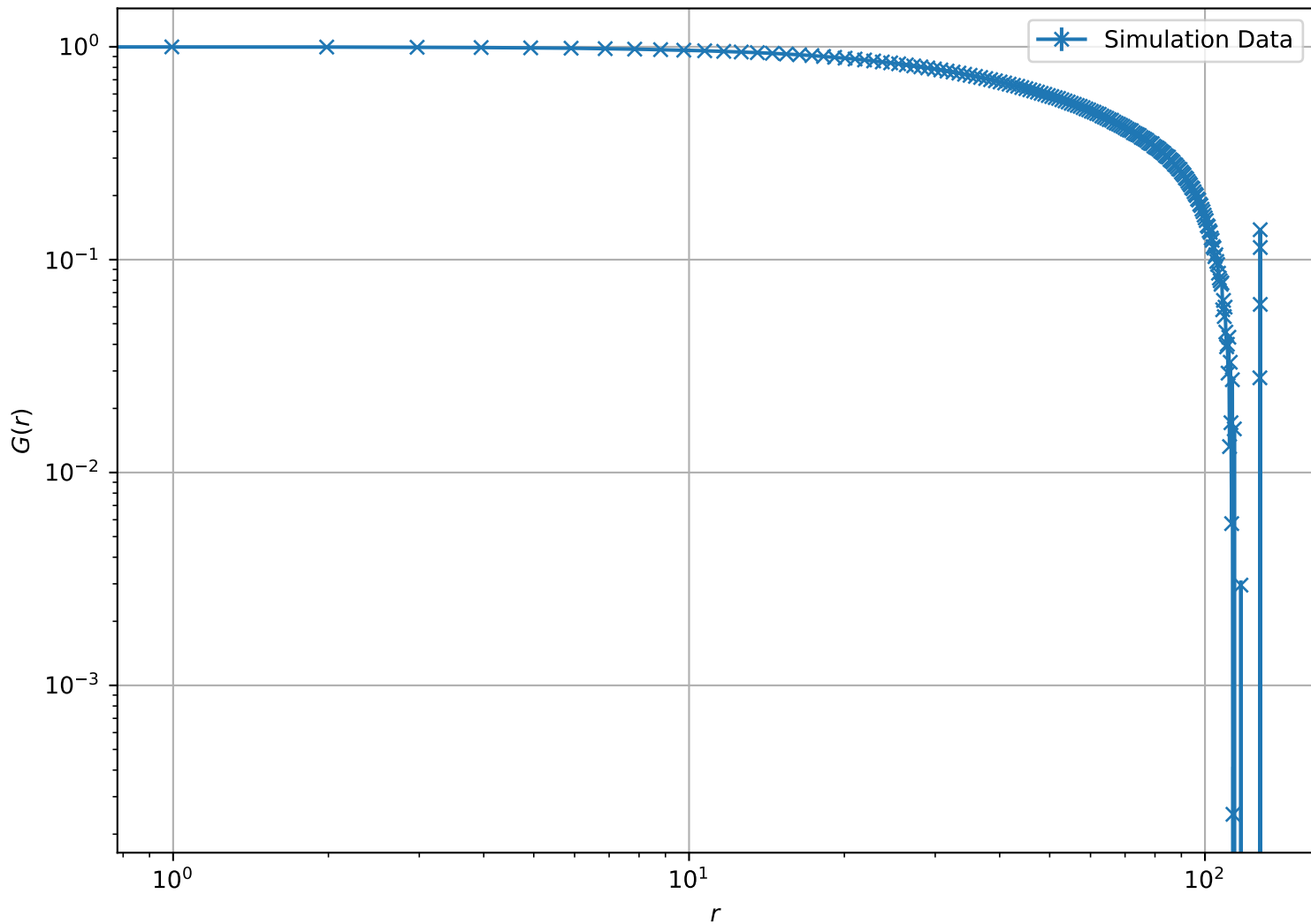
Correlation Function at T = 1.00e - 05 , L = 128 (Log-Log Scale)
