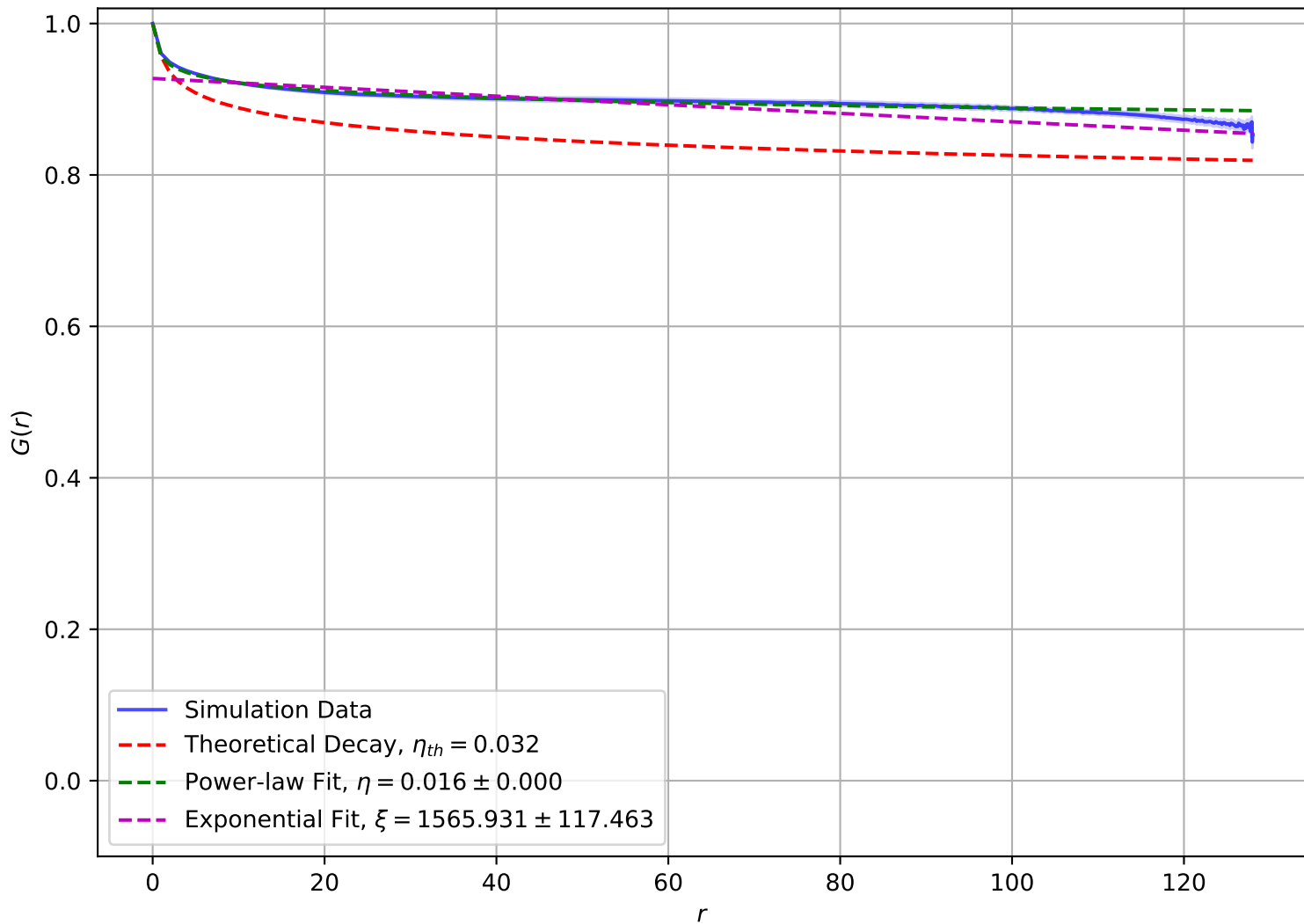
Correlation Function at T = 2.00\text{e} - 01 , L = 128
