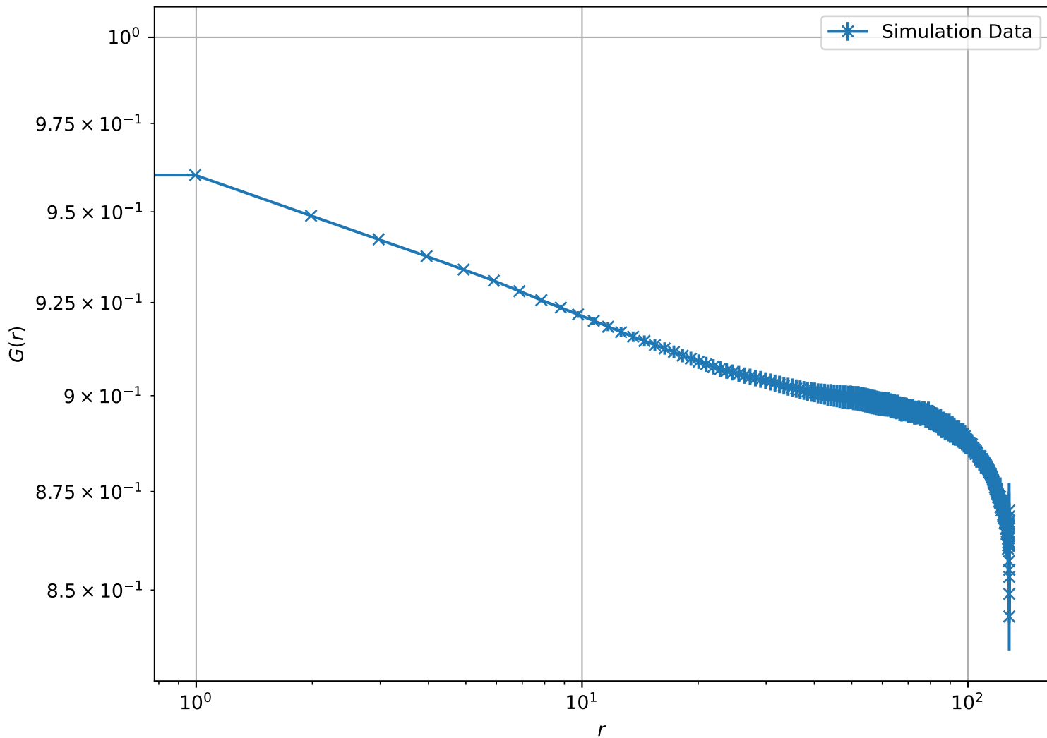
Correlation Function at T = 2.00e - 01 , L = 128 (Log-Log Scale)
