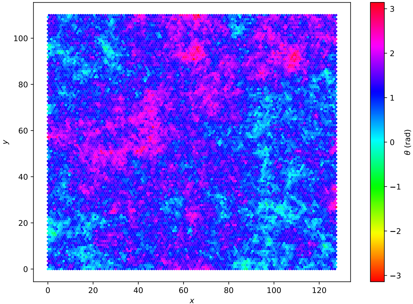
Hexagonal Lattice L=128 , T = 4.00e - 01
