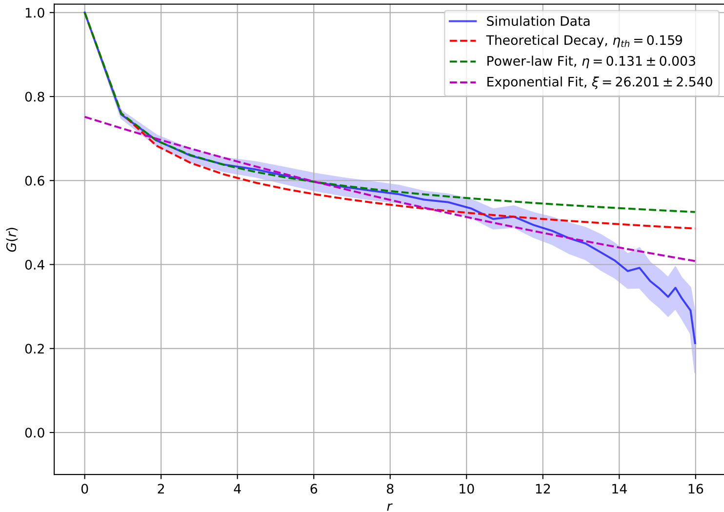
Correlation Function at T = 1.00e + 00 , L = 16
