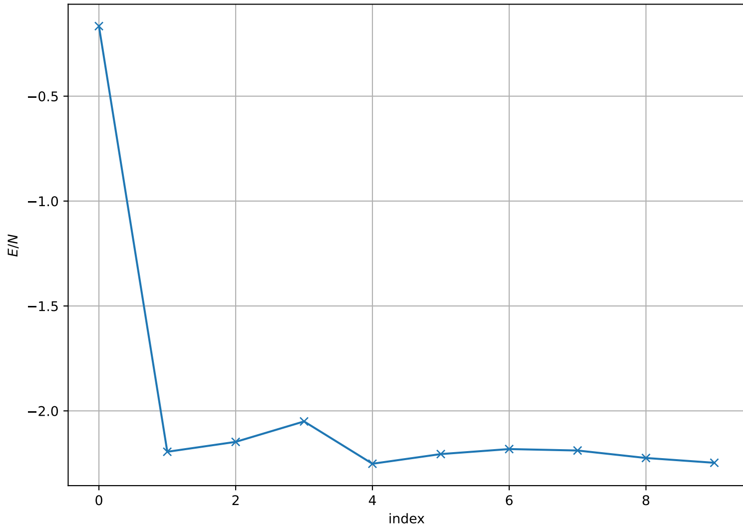
Energy per Site at T = 1.000e + 00 , L = 16
