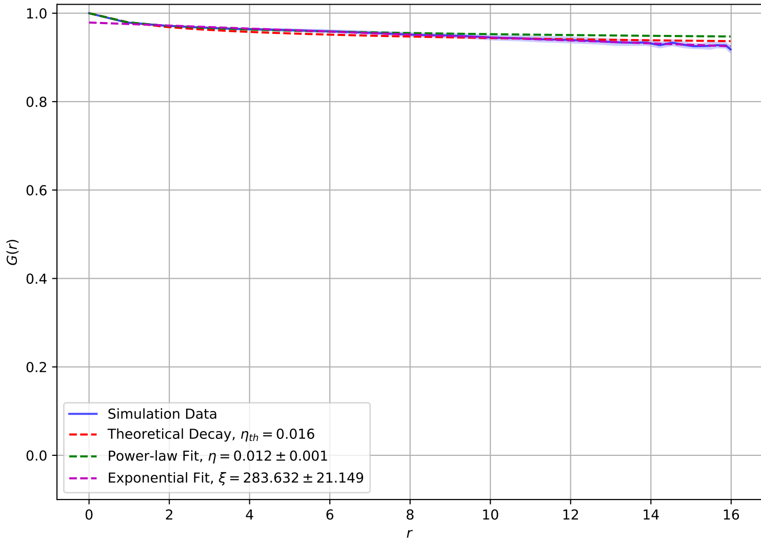
Correlation Function at T = 1.00e - 01 , L = 16
